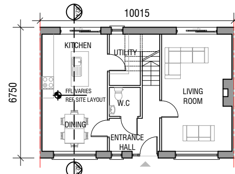
B2.4 GROUND FLOOR PLAN SCALE 1:200 NORTH POINT VARIES REFER TO SITE LAYOUT PLAN
