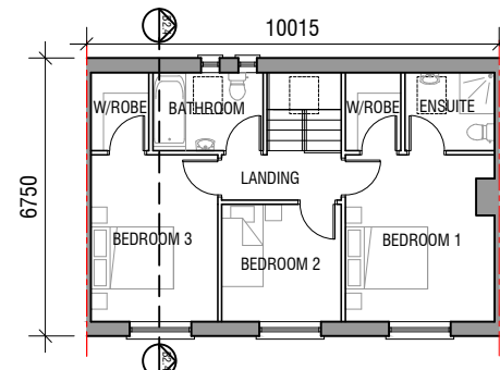
B2.4 FIRST FLOOR PLAN SCALE 1:200 NORTH POINT VARIES REFER TO SITE LAYOUT PLAN
