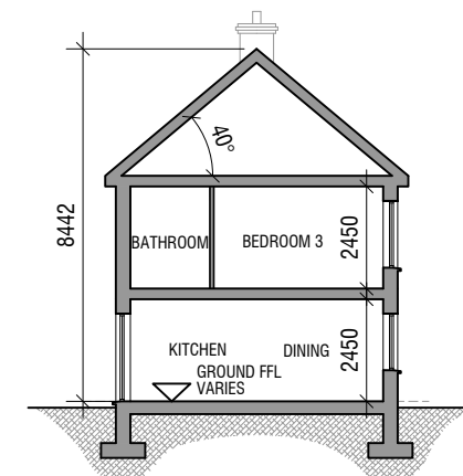
SECTION B2.4 SCALE 1:200
