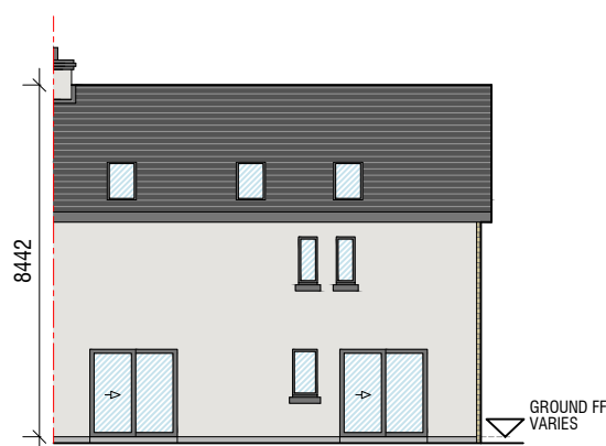
B2.3 REAR ELEVATION SCALE 1:200 GROUND FFL VARIES
