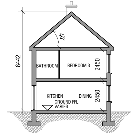
SECTION B2.3 SCALE 1:200
