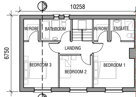
B2.3 FIRST FLOOR PLAN SCALE 1:200 NORTH POINT VARIES REFER TO SITE LAYOUT PLAN
