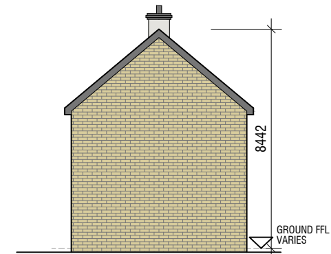
B2.3 LHS ELEVATION SCALE 1:200 GROUND FFL VARIES
