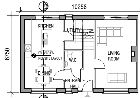
B2.3 GROUND FLOOR PLAN SCALE 1:200 NORTH POINT VARIES REFER TO SITE LAYOUT PLAN
